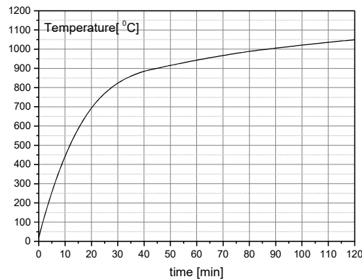
Figure 1. The Standard time / temperature curve in ISO 834
