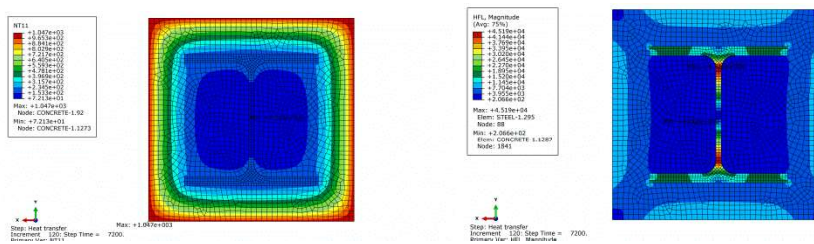
Figure 5. Temperature and heat flux fields of HEB 260 composite steel-concrete column of square cross section after 120min of fire onset
