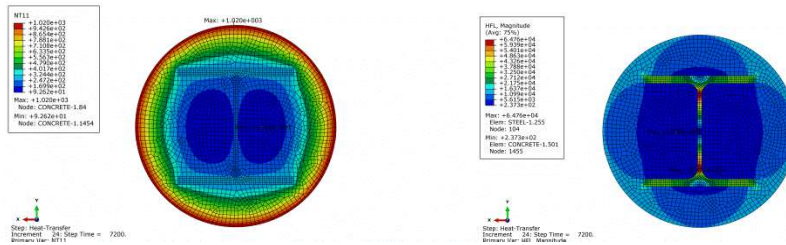
Figure 4. Temperature and heat flux fields of HEB 260 composite steel-concrete column after 120min of the fire exposure
