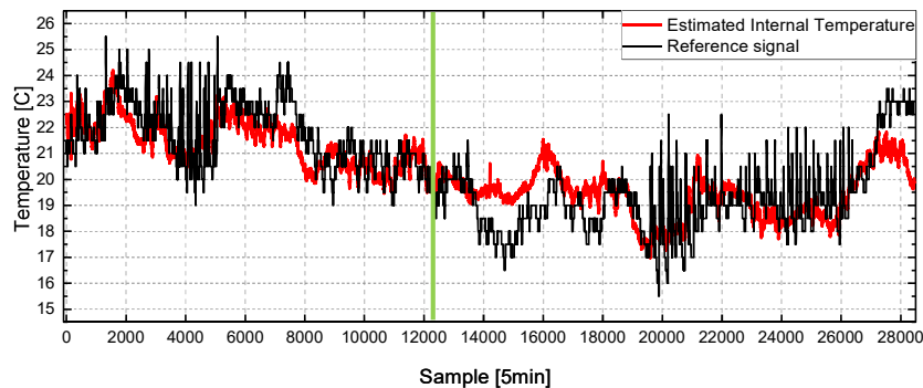
Figure 7. Estimated exterior near-wall air temperature \tilde{T}_i
