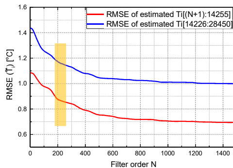
Figure 5. RMSEs for temperature estimations for the filter order ranging from 1 to 1500.
