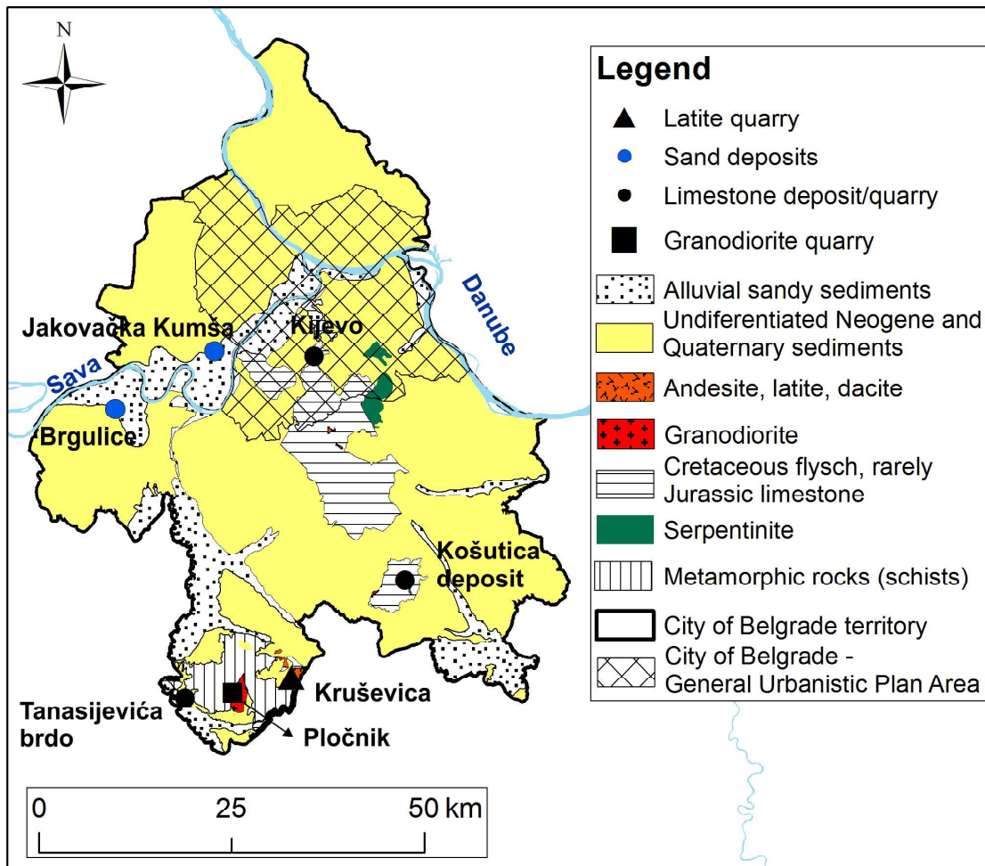
Fig. 1. Geological map of Belgrade with position of existing aggregate quarries and sand pits (after Basic Geologic Map of SFRJ, sheets Beograd, Pančevo, Obrenovac, Smederevo and Kragujevac).
