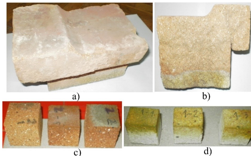
Figure 1. The visual appearance of the sample from the furnace wall: a) sample, b) section of the sample with the appearance of positions I and II, c) Position I, and d) Position II.
