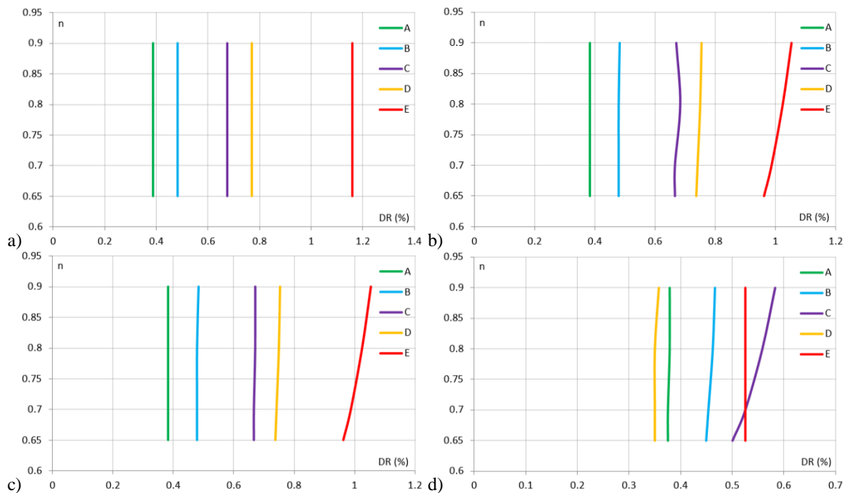
Figure 3. Variation of the global drift for the level of target displacement in the function of different types of soil A, B, C, D and E – introduction of KIE: a) e=0 , b) e=3m , c) e=9m , d) e=15m
