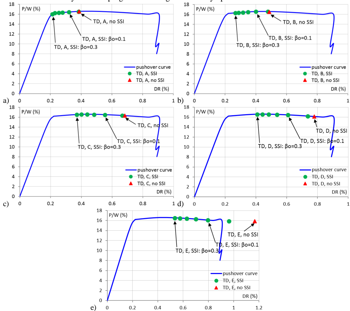
Figure 5. NSPA pushover curves and target displacements (TD) for soil types: a) A, b) B, c) C, d) D, e) E
