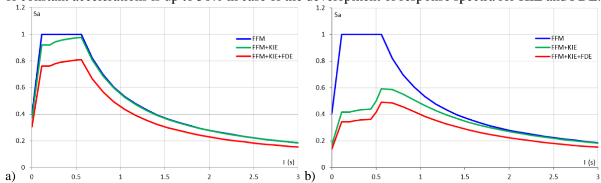
Figure 2. Diagrams of elastic response spectra for FFM, response spectra corrected by KIE and response spectra corrected with KIE and FDE for type C soil, v_s=600\text{m/s}^2 , \beta_0=0.05 : a) e=0 , b) e=9 m
